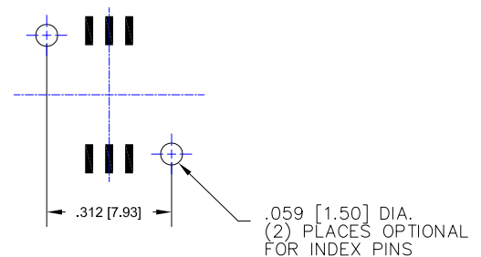
FOOTPRINT LAYOUT TOP VIEW
