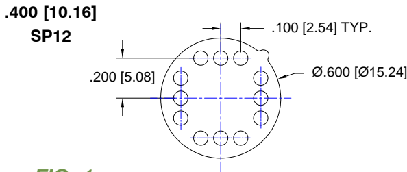
FIG: 1 Thru-Hole: R400-SP12-02T-01S-R27-L14 Surface Mount: R400-SP12-02T-93S-R27-L14
